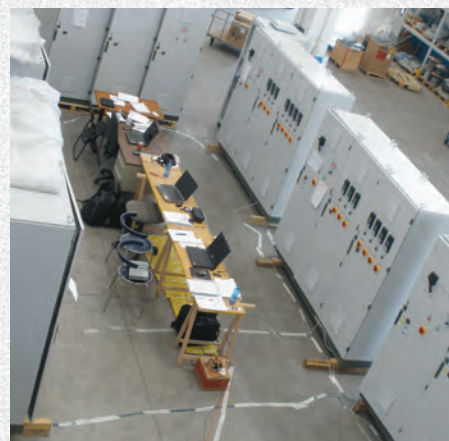
COLLAUDO IN SEDE Factory test
